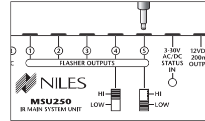
FIGURE 3 Connecting the MicroFlasher to the main system unit's flasher low outputs.
